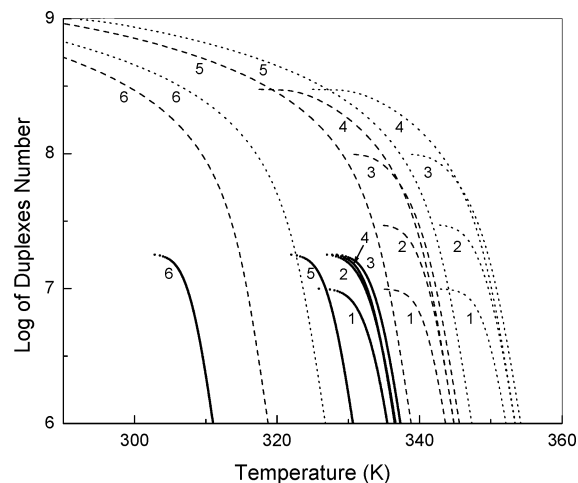
Figure 1. Number of hybrids vs temperature for the assayed target concentrations 10^{-12} (solid), 10^{-9} (dashed), and 10^{-6} mol/L (dotted). The numbers denote the probe surface density: (1) 10^{11} , (2) 3 \times 10^{11} , (3) 10^{12} , (4) 3 \times 10^{12} , (5) 10^{13} , and (6) 3 \times 10^{13} \text{ cm}^{-2} .
